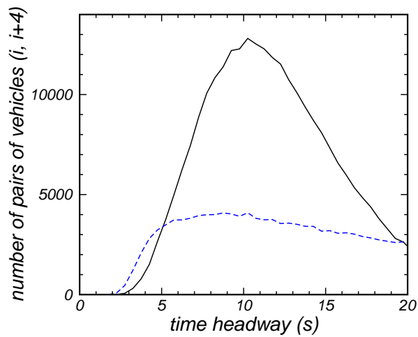
FIG. 2: (Color online) Distribution of time headways between vehicles of rank i and i+4 , on the right-slow lane (black solid line) and on the left-fast lane (grey — blue online — dashed line).
