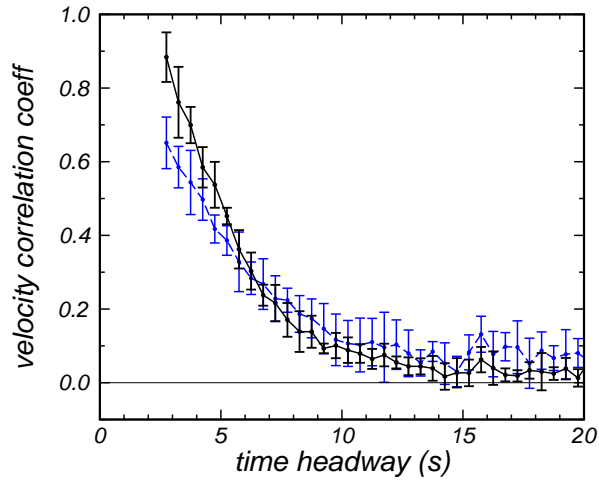
FIG. 3: (Color online) For pairs of vehicles of rank i and i+4 : Velocity correlation coefficient as a function of the time headway, on the right-slow lane (black solid line) and on the left-fast lane (grey — blue online — dashed line).
