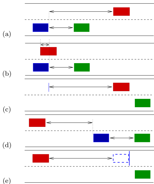
FIG. 5: (Color online) Schematic representation of the inter-lane time headway measurements, for a two-lane road. Vehicles are driving to the right. In Fig. (a), a time headway shorter than 0.5s separates the two vehicles on the right lane. Then, the time headway between the right lane following car and its predecessor on the other lane is computed as indicated by the arrow (in all the schemes, a spatial representation has been substituted to the temporal one, though in practice, one computes the passage time difference between the rear of the left lane vehicle and the front of the right lane vehicle). Fig. (b) illustrates how a negative time headway can be obtained : the front of the left lane vehicle went first on the magnetic loop (thus it is the leader of the right lane vehicle), but its rear arrived on the loop after the front of the right lane vehicle. Fig. (c), the time headway is computed between a virtual vehicle whose location is randomly chosen, and its predecessor on the same (left) lane. The procedure is independent of the right lane state. Fig. (d): same as (a), but it is the successor that is considered on the left-lane. Fig. (e): same as (c), but the time headway is computed with the successor of the virtual vehicle. The ratio length/velocity of the virtual vehicle is chosen randomly according to the distribution of length/velocity ratios of the right-lane vehicles.
