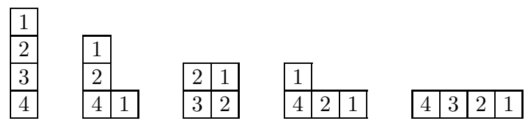
Fig. 2. partitions of 4 and the hook lengths h_v
