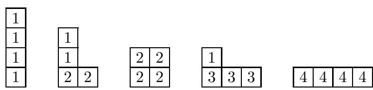
Fig. 3. partitions of 4 and the part lengths p_v
