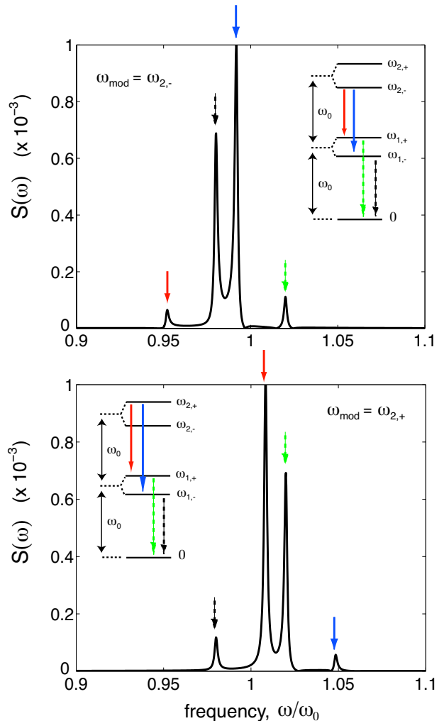
FIG. 3: Spectrally resolved emission per unit time for given values of the modulation frequency: \omega_{\text{mod}} = \omega_{2,-} (top panel), \omega_{\text{mod}} = \omega_{2,+} (bottom panel). The modulation amplitude is \Delta g/\gamma = 0.1 . The insets illustrate the optical transitions responsible for the different emission lines that are visible in the main panels. For the sake of clarity, the level spacings in the insets are not in scale.
