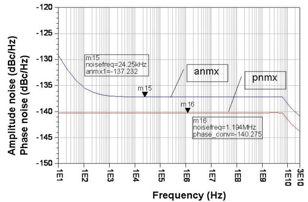
Fig. 6 Simulated optical link phase noise and amplitude noise around the RF carrier (10 GHz)
