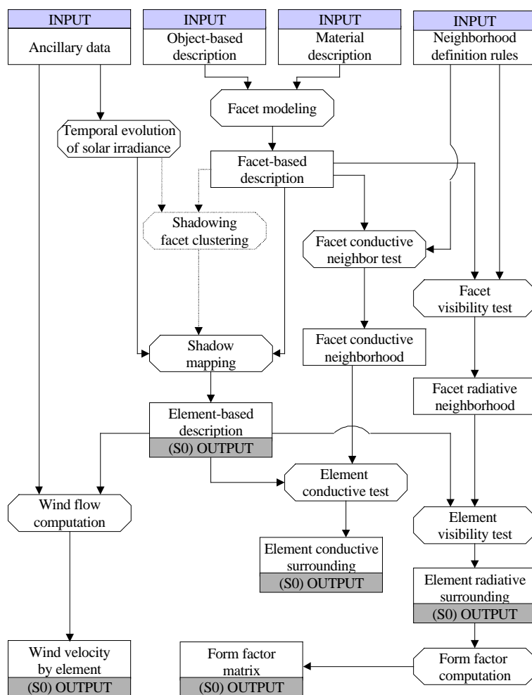
Figure 5: the detailed architecture of the (S0) primary simulator. In full lines, the required architecture to obtain elements; in dotted lines, the shadowing facet clustering, giving the opportunity to accelerate and to optimize the element creation.
