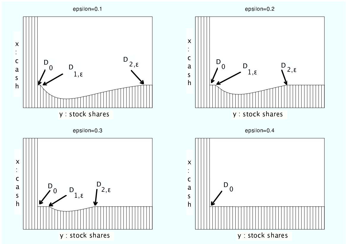
Figure 4: Domain \mathcal{S}_\epsilon in the nonhatched zone for fixed p = 1 and \theta = 1 and \epsilon evolving from 0.1 to 0.4. Here \kappa_b = 0.9 and f(e, \theta) = \kappa_b \exp\left(\frac{e}{\theta}\right) for e < 0 . Notice that for \epsilon large enough, \mathcal{S}_\epsilon is equal to open orthant \mathbb{R}_+^* \times \mathbb{R}_+^* .
