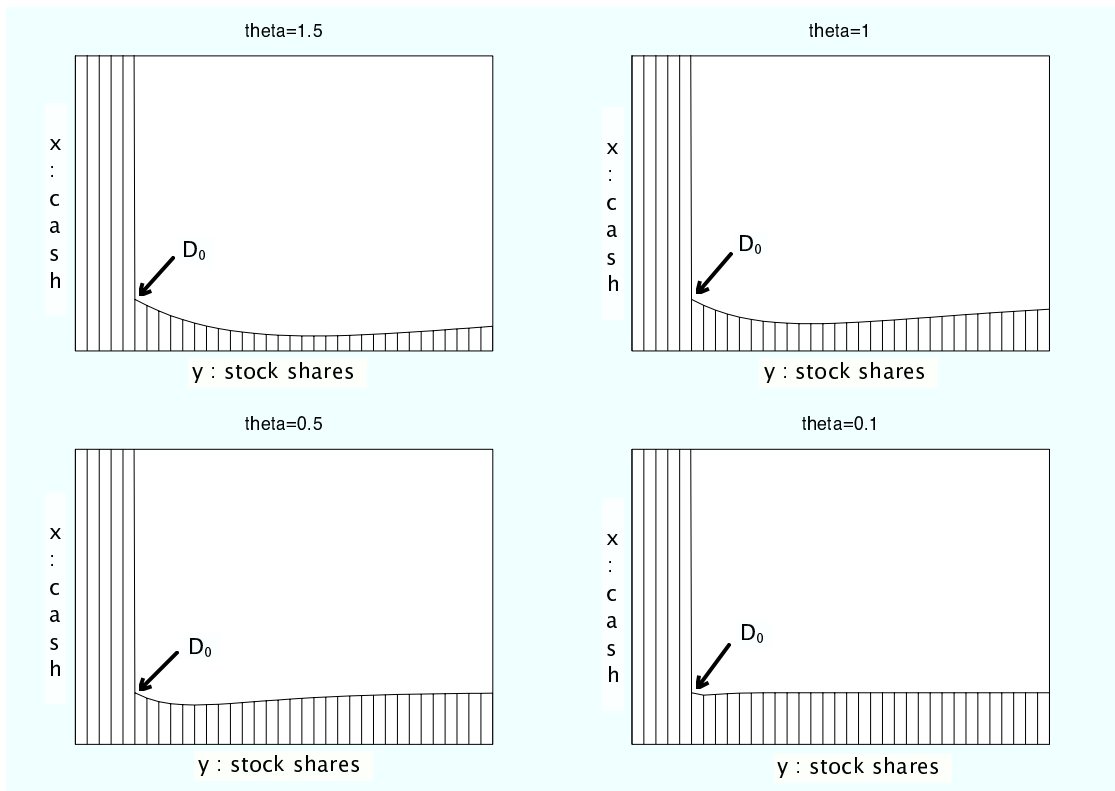
Figure 1: Domain S in the nonhatched zone for fixed p = 1 and \theta evolving from 1.5 to 0.1. Here \kappa_b = 0.9 and f(e, \theta) = \kappa_b \exp(\frac{e}{\theta}) for e < 0 . Notice that when \theta goes to 0, the domain converges to the open orthant \mathbb{R}_+^* \times \mathbb{R}_+^* .
