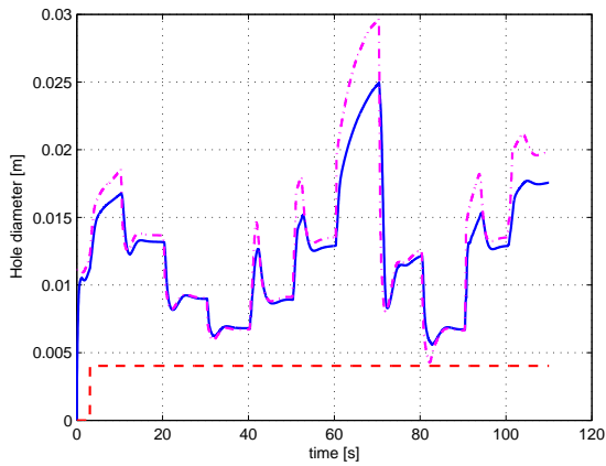
Fig. 9. 4mm Hole - Hole estimation in solid line and variable thresholds are dot dashed when \epsilon_{exh} = 150mbar and M_{exh} = 200mbar . Reference hole diameter is dashed.
