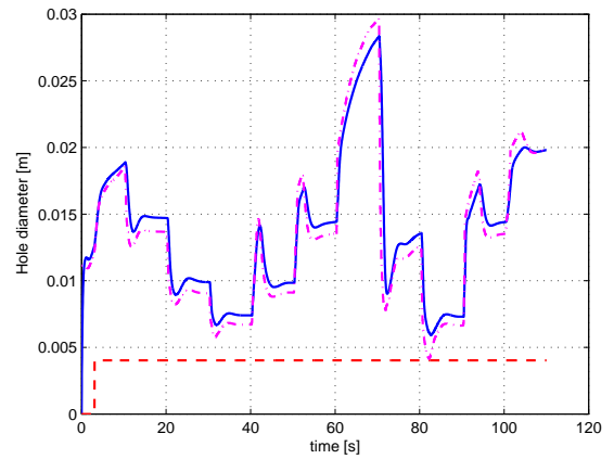
Fig. 8. 4mm Hole - Hole estimation in solid line and variable thresholds is dot dashed when \epsilon_{exh} = 200mbar and M_{exh} = 200mbar . Reference hole diameter is dashed.
