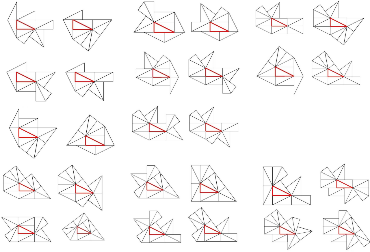
Figure 3: 28 collared prototiles.
