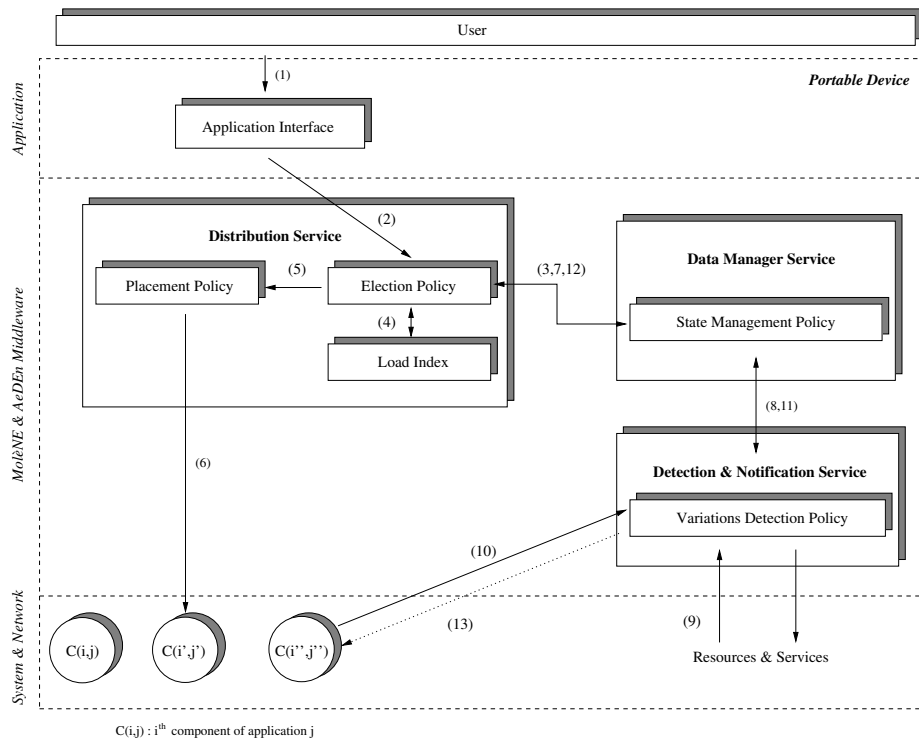
Figure 2. AeDEN architecture
