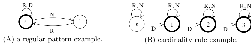
Fig. 4. Examples of automata representing work regulations.
