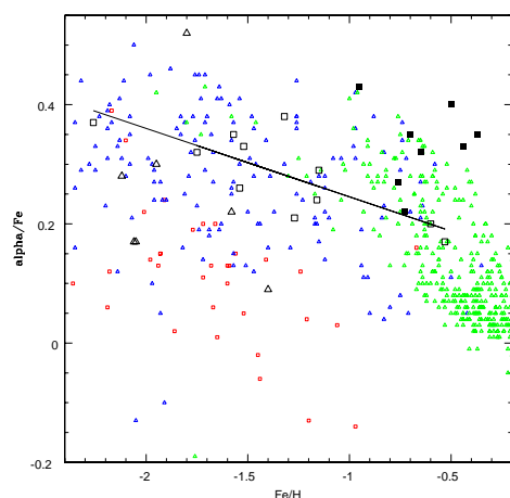
Figure 5. Metallicity versus light-element abundance. Same symbols as previous figures. The line is a least-squares fit to the globular clusters of group 1. Small triangles are disc (green) and halo (blue) field stars. Small red open squares are dwarf galaxies of the Local Group (from Venn et al. 2004)
