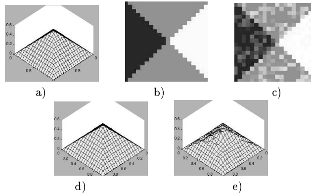
Fig. 4. Results for a synthetic image generated by a pyramidal surface sampled on a grid of size 20 \times 20 with \theta = 36^\circ : a) original surface, b) original image, c) noisy image; d) surface reconstructed from b): n = 89 , \epsilon_1 = 0.4\% , \epsilon_2 = 0.4\% , \epsilon_\infty = 0.8\% ; e) surface reconstructed from c): n = 91 , \epsilon_1 = 23.7\% , \epsilon_2 = 23.2\% , \epsilon_\infty = 26.3\% .
