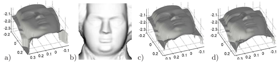
Fig. 5. a) original surface; b) image generated from a) [size \simeq 200 \times 200 ]; c) reconstructed surface from b) with the implicit algorithm (IA) after only 3 iterations, using the exact boundary data at all critical points and with state constraints on the boundary of the image: \epsilon_1 \simeq 0.58 , \epsilon_2 \simeq 0.0019 , \epsilon_\infty \simeq 0.42 ; d) reconstructed surface by the IA (after 3 iterations) with state constraints on the boundary of the image and at all the critical points except at that on the nose: \epsilon_1 \simeq 0.60 , \epsilon_2 \simeq 0.0020 , \epsilon_\infty \simeq 0.42 .
