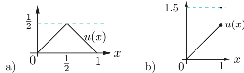
Fig. 2. a) Continuous viscosity solution of (2) with u(0) = u(1) = 0 ; b) discontinuous viscosity solution of (2) with u(0) = 0 and u(1) = 1.5 .
