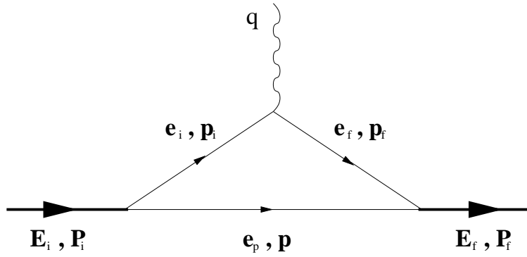
Figure 1: Graphical representation of a virtual photon absorption on a pion together with kinematical definitions.
