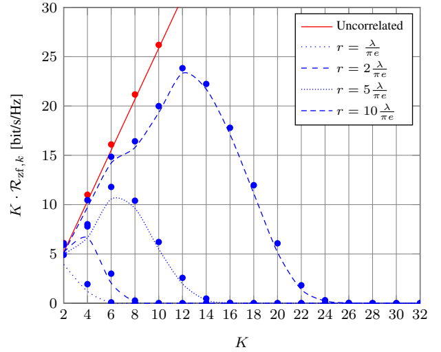
Fig. 2. ZF, UCA, Ergodic MIMO sum rate K \cdot \mathcal{R}_{\text{zsf},k} for different r/\lambda , \beta = 1.5 , 1/\sigma^2 = 10 dB, numerical simulations indicated by circle marks
