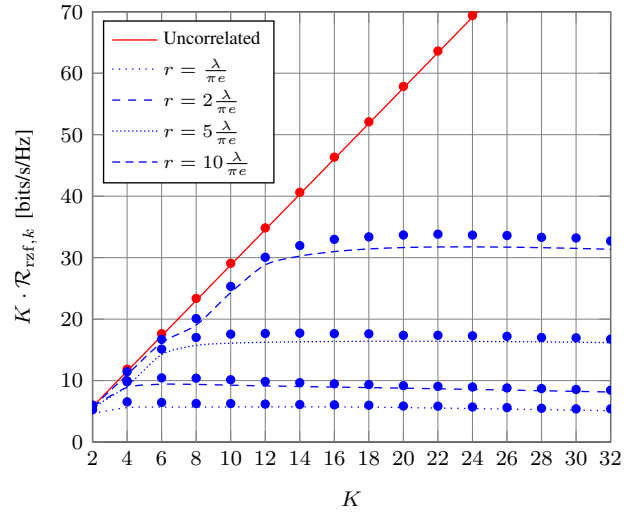
Fig. 3. R-ZF, UCA, Ergodic MIMO sum rate K \cdot \mathcal{R}_{\text{zsf},k} for different r/\lambda , \beta = 1.5 , 1/\sigma^2 = 10 dB, numerical simulations indicated by circle marks
