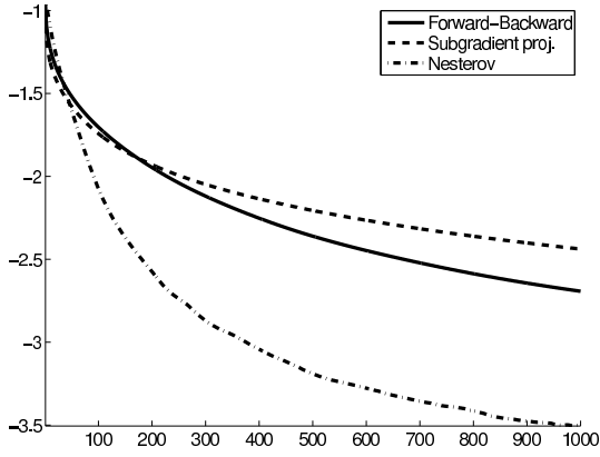
Fig. 3. Decay with k of the total variation error \log_{10}(\|f^{(k)}\|_{\text{TV}}/\tau - 1) for the same algorithms as in Figure 2. Here \tau = \|f_0\|_{\text{TV}}/4 .
