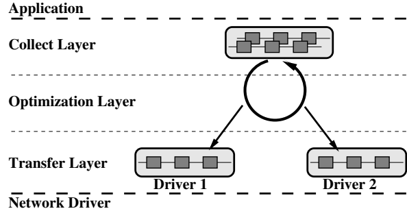
Figure 4. Fine grain locking in NEWMADELEINE
