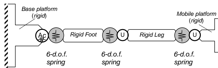
Fig. 3. Flexible model of a single kinematic chain (Ac – actuating joint, U – universal joint)
