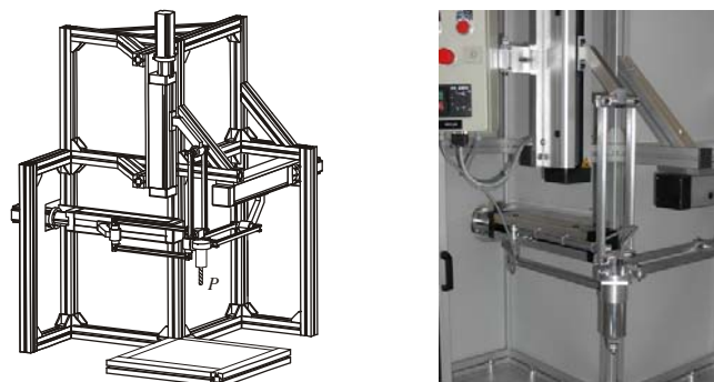
Fig. 6. CAD model of and Orthoglide and its prototype
