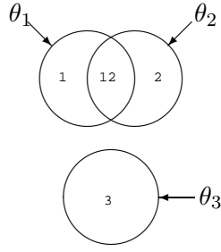
Fig. 3: Venn diagram of a DSm hybrid model for a 3D frame.
