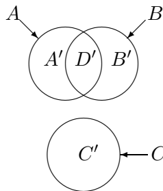
Fig. 4: Hybrid model for \Theta = \{A, B, C\} .
