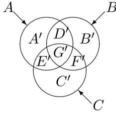
Fig. 5: Free DSMP model for a 3D frame.
