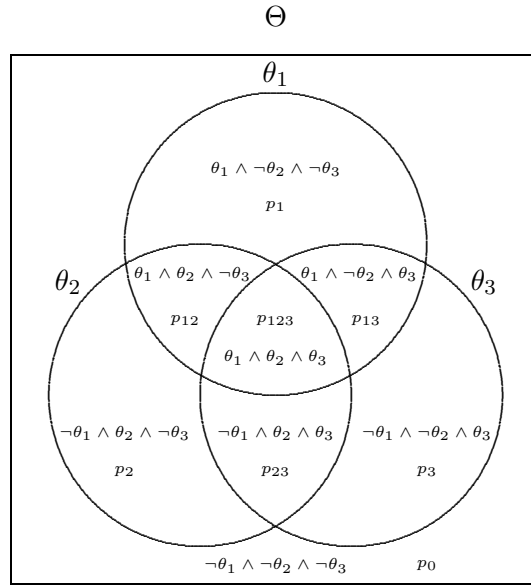
Fig. 2: Venn diagram of the free DSsm model for a 3D frame.
