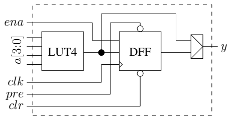
Fig. 1. Minimal structure used in our vendor neutral flow, corresponding to the common denominator of usual FPGAs.
