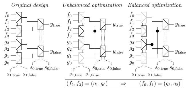
Fig. 5. Optimization B incorrectly (since partially) and correctly implemented on a redundant design.
