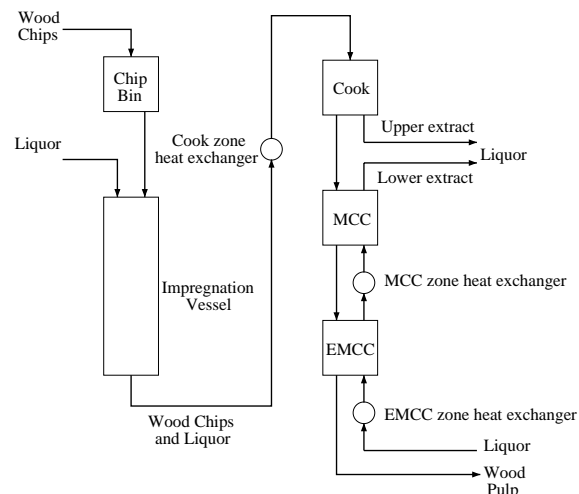
Fig. 1. Schematic of a chemical pulp digester.
