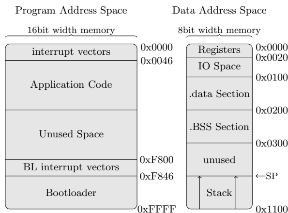
(b) Typical memory organisation on an Atmel Atmega 128. Program memory addresses are addressed either as 16bit words or as bytes depending on the context.
