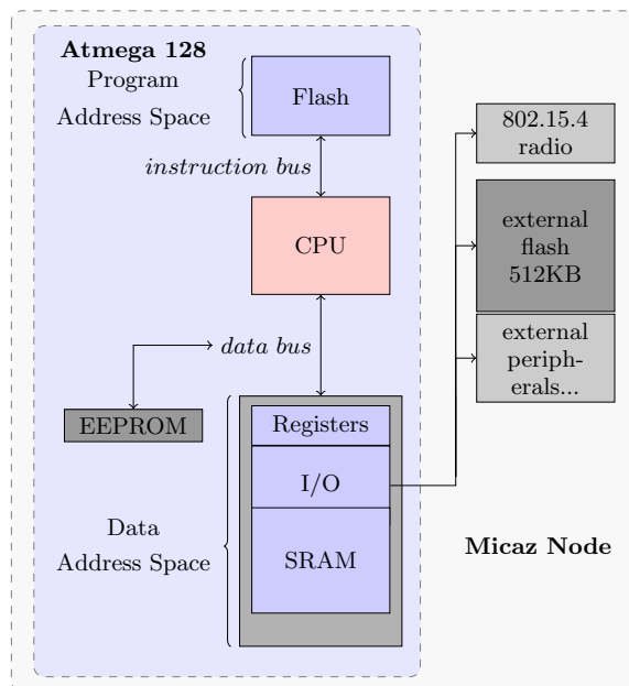
(a) Micaz memory architecture putting in evidence the physical separation of memory areas, on top of the figure we can see the flash memory which contains the program instructions.
