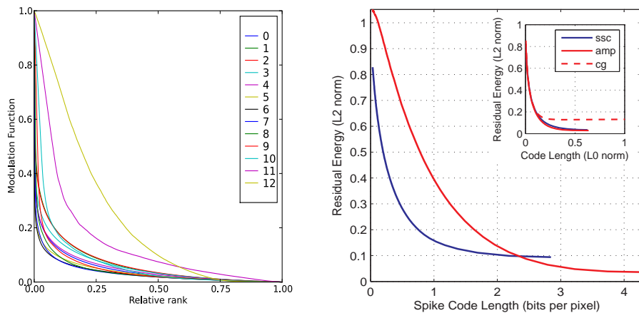
Figure 4: Efficiency of Competition Optimized Matching Pursuit (COMP). Spike Coding and Sparse Spike Coding (using COMP) produce flows of spikes representing the image. By representing the the distance of the original image with a reconstruction, one may quantify the dynamical efficiency of this solution as a function of the number of spikes. ( Left ) When applying the algorithm on a set of natural images, the coefficients exhibited differences in their probability density functions. We show this by plotting the cumulative density functions of the coefficients for different levels in the pyramid. Using these cumulative pdf, one could transform the pyramids of coefficients in pyramids for which all coefficients where a priori equiprobable. This optimizes the ArgMax operator which is at the heart of the Sparse Spike Coding scheme. ( Right ) The resulting COMP solution gives a similar result than MP in terms of residual energy as a function of pure L_0 sparseness (see inset). In fact, in MP, by taking the maximum absolute, and since the decrease of energy is proportional to the square of the coefficient (see Chapter 3.1.2 of (Perrinet, 2007)) one ensures that the decrease of MSE per coefficient is optimal for MP. These are both better for that purpose than conjugate gradient. However, when defining the efficiency in terms of the residual energy as a function of the description length of the spiking code word, then the proposed COMP model is more efficient than MP because of the quantization errors inherent to the higher variability of coded coefficients. Thus, including homeostasis improved the efficiency of adaptive Sparse Spike Coding by ensuring that the decrease of MSE per bit of code is optimal. It should be noted that the homeostasis mechanism is important during “learning” but that it is not useful for “pure” coding (see Sec. 5).
