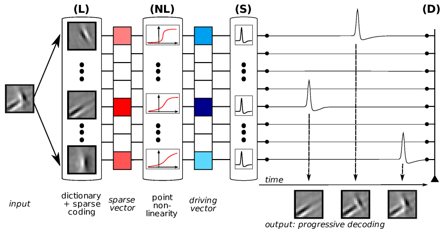
Figure 3: Spike Coding of natural images. We did build here a simple framework of pyramidal neurons illustrating the efficiency of neural architectures compared to classical computer architectures. We show here how a bundle of L-NL neurons (Carandini et al., 1997, 2005) tuned by a simple homeostatic mechanism allow to transfer a transient information, such as an image, using spikes. (L) The signal to be coded, for instance the match \rho_j of an image patch (the tiger on the left bottom) with a set of filters (edge-like images), may be considered as a stochastic vector defined by the probability distribution function (pdf) of the values \rho_j to be represented. (NL) By using the cumulative function as a point non-linearity f_j , one ensures that the probability of z_j = f_j(\rho_j) is uniform, that is that the entropy is maximal. This non-linearity in the L-NL neuron implements a homeostasis that is controlled only by the time constant with which the cumulative probability function f_j is computed (typically 10^4 image patches in our case). (S) Any instance of the signal may then be coded by a volley of spikes: a higher value corresponds to a shorter latency and a higher frequency. (D) Inversely, for any spike events vector, one may estimate the value from the firing frequency, the latency. We may simply use the ordering of the spikes since the rank provides an estimate of the quantile in the probability distribution function thanks to the equalization. Using the inverse of f_j one retrieves the value in feature space so that this volley of spikes is decoded (or directly transformed) thanks to the relative timing of the spikes using the modulation (see Eq. 10). This builds a robust information channel where information is solely carried by spikes as binary events. Given this model, the goal of this work is to find the most efficient architecture to code natural images and in particular to define a coding cost and to derive efficient compression algorithms. Note that this scheme is similar to the N-NL scheme but that instead of generating a Poisson point process, we use the exact timing. This is allowed by the point non-linearity which permits to code the value by the timing and not the firing frequency.
