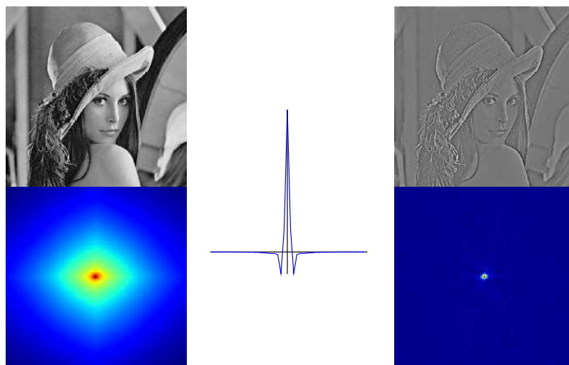
Figure 1: Spatial decorrelation. ( Top-Left ) Sample raw natural image ( M = 512^2 ). ( Bottom-Left ) Mean pairwise spatial correlation in a set of 1000 natural images (Red is 1, blue is zero). It shows the typical decrease in \frac{1}{f^2} of the power spectrum but also an anisotropy along the vertical and horizontal axis. ( Middle ) decorrelation filter computed from the methods of (Atick, 1992) (see text). This profile is similar to the interaction profile of bipolar and horizontal cells in the retina. ( Top-Right ) Whitening of the sample image. ( Bottom-Right ) The mean pairwise spatial correlation of 1000 whitened natural images is highly peaked at the origin and inferior to 0.05 elsewhere. As is observed in the LGN, the power spectrum is relatively decorrelated by our pre-processing (Dan et al., 1996). See script experiment.whitening.py to reproduce the figure.
