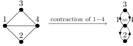
FIGURE 6. Example of contraction.
