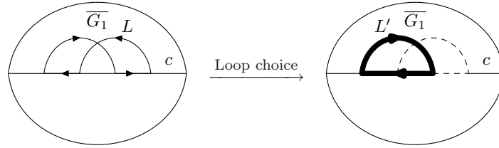
FIGURE 20. Good choice of cycle
