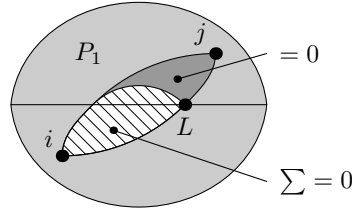
FIGURE 25. Case 1: i \notin V_c and j is not in the same region than i .
