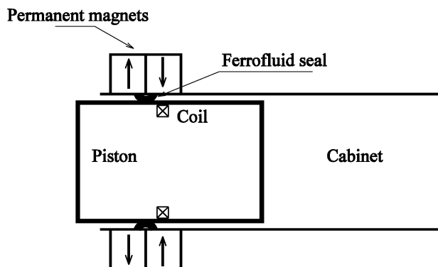
Fig. 1. Loudspeaker principle.
