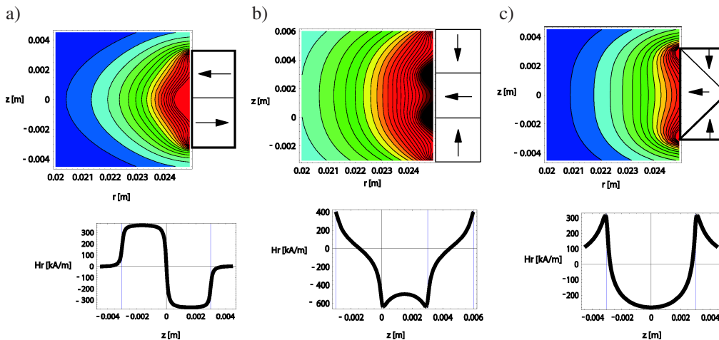
Fig. 3. Various magnet assemblies: a) two magnets, b) three magnets: rectangle, c) three magnets: triangle.
