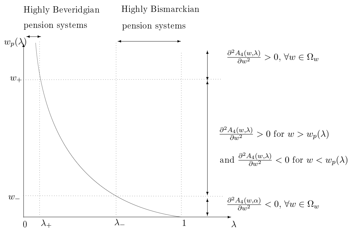
Figure 6.4: Illustration of lemma 3
