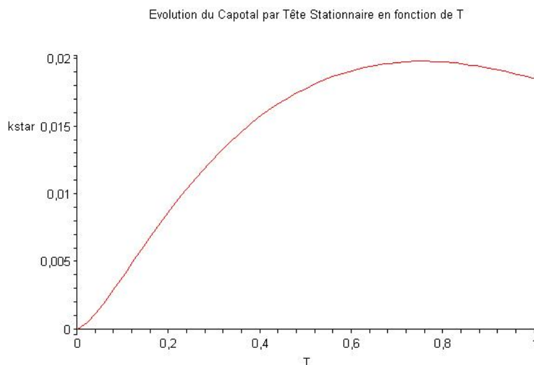
Figure 1.3: k in function of T for n = 0.1 .
