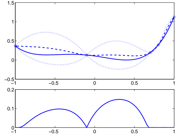
Figure 3. Illustration of a kriging interpolation and corresponding EI. Top: similarity function of one variable (continuous line), observations (circles), kriging prediction (dashed line), uncertainty – related to the predicted kriging error (dotted line). Bottom: the expected improvement. Note that the maximizer of the EI and the minimizer of the interpolation are not necessarily the same.
