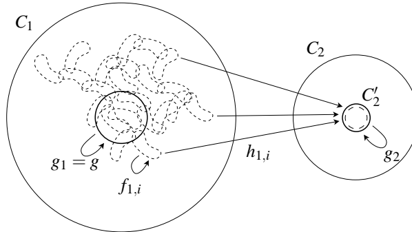
Figure 3: Fragment and push every piece inside the small disc...
