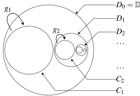
Figure 1: Construction of g
