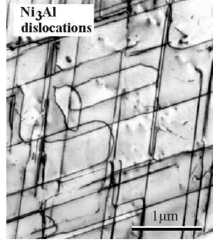
Figure 1: Dislocation lines in Nickel Aluminium alloy.
