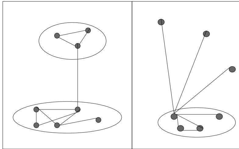
Figure 6 : Structural Holes
