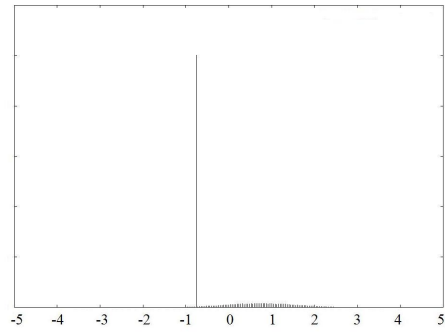
(D.a) \Delta(0, 1, 3(\sqrt{6}-2)\sqrt{3-\sqrt{6}}, 0)
