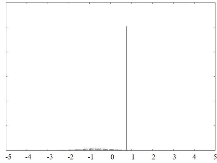
(D.b) \Delta(0, 1, -3(\sqrt{6}-2)\sqrt{3-\sqrt{6}}, 0)
