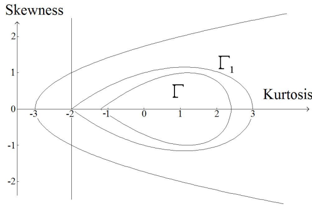
Figure 3.1: Sets of admissible couples \Gamma and \Gamma_1
