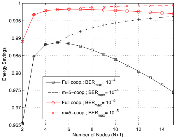
Fig. 2. The average energy savings curves versus the number of transmitting nodes, (N + 1) , employing full-cooperation and m -cooperation with two different BER_{max} constraints.
