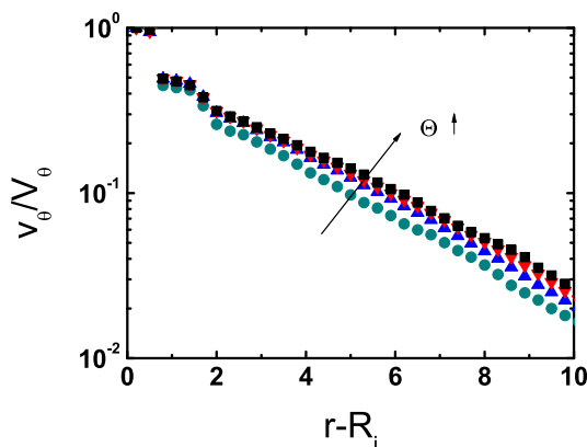
FIG. 21: (Color online) Velocity profiles v_\theta(r)/V_\theta for different values of \Theta (rad). (●) \Theta = \pi/16 , (▲) \Theta = \pi/8 , (▼) \Theta = \pi/2 , (■) \Theta = 2\pi . R_i = 25 , R_o = 50 , V_\theta = 2.5 .
