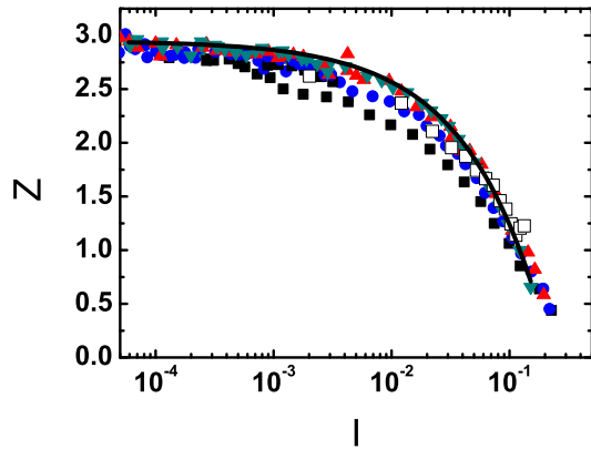
FIG. 13: (Color online) Coordination number Z as a function of the inertial number I (the solid line represents the function Z = 2.95 - 7.65I^{0.65} ) for different geometries. (■) R_{25} , (●) R_{50} , (▲) R_{100} , (▼) R_{200} , (□) plane shear [4]. V_\theta = 2.5 .
