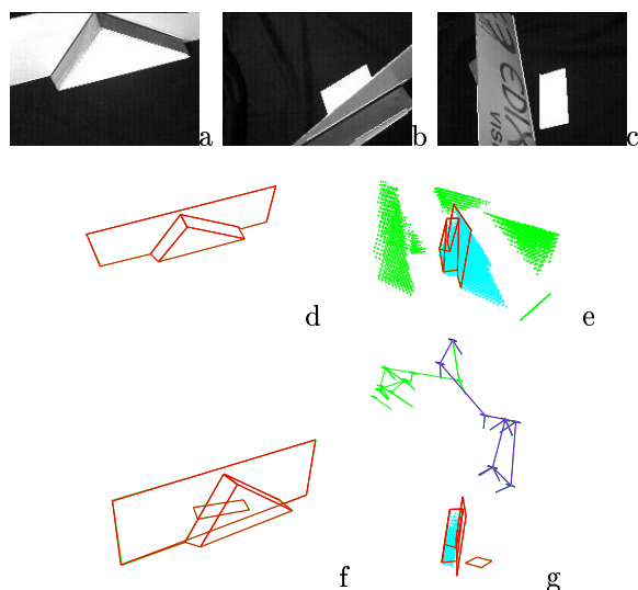
Fig. 17. Polyhedral scene reconstruction: (a) First image of the scene acquired by the camera, (b) detection of a new polygon during the exploration process, (c) detection of the last primitive, (d) Reconstructed model of the scene after the first local exploration process, (e) unobserved and occluded areas (56% of the scene has been already observed), (f) final reconstructed model of the scene, (g) camera trajectory and residual area (99.2% of the scene has been observed).
