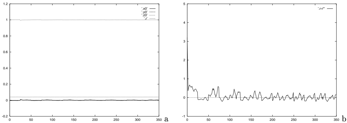
Fig. 13. Estimation of the parameters of a cylinder: (a) estimated position of a point on the axis ( x_0, y_0, z_0 ) and radius r (in mm), (b) error between the real and estimated radius of the cylinder (in mm)
