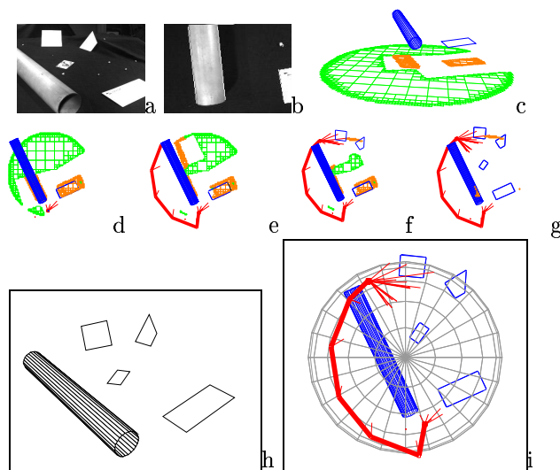
Fig. 18. Cylinder and polygons reconstruction (a) External view, (b) first view of the scene and results of the first incremental reconstruction process, (c) reconstructed scene and projection on a virtual plane of the unknown area, (d-g) different steps of the global exploration process (camera trajectory, 3D model of the reconstructed scene and projection on an virtual plane of the unknown area), (h) 3D model of the reconstructed scene, (i) polar view of the camera trajectory.
