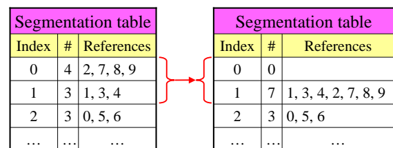
Figure 3: The segment with index 0 in the segment table is merged with the segment indexed 1 by moving the indices of the DEM points in segment 0 to the reference list of segment 1.
