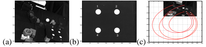
Figure 4: Initial -a-, desired -b- images of the target and trajectories planned without repulsive potential -c-
