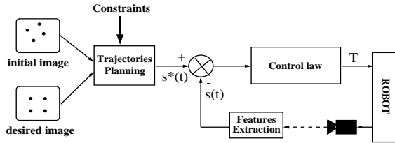
Figure 1: Block diagram of the method
