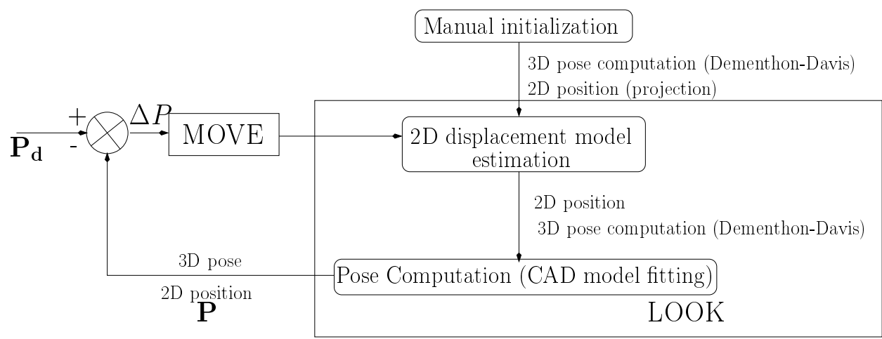
Figure 12: Overview of the visual servoing task.
