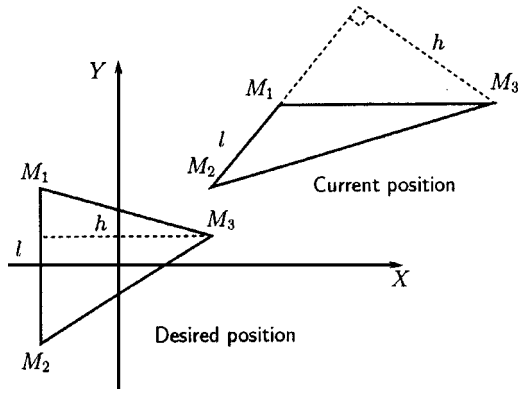
Fig. 5. Triangle built from three feature points of the object.
