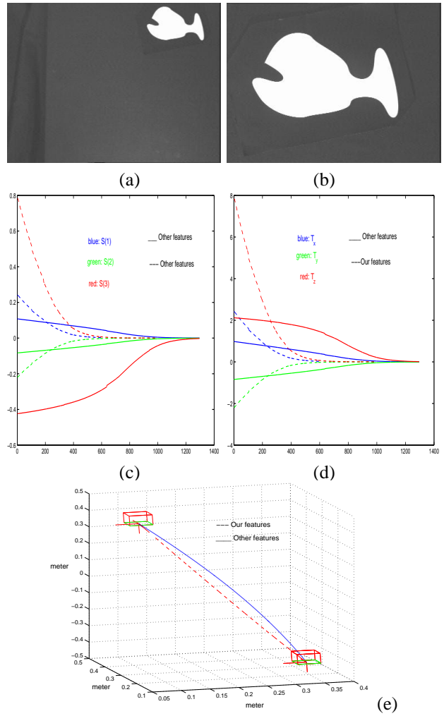
Fig. 2. Results for a pure translational motion: (a) initial image, (b) desired image, (c) visual features (\mathbf{s} - \mathbf{s}^*) , (d) camera velocity \mathbf{T}_C , (e) camera 3D trajectory
