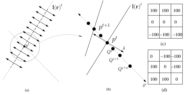
Figure 2. Determining points position in the next image using the ME algorithm: (a) calculating the normal at sample points, (b) sampling along the normal (c-d) 2 out of 180 3x3 predetermined masks (in practice 7x7 masks are used) (c) 180° (d) 45°.
