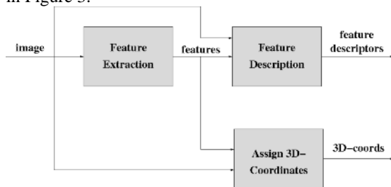
Figure 3: Object Recognition: Off-line training
