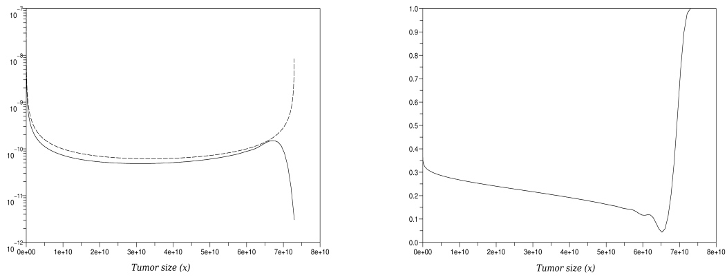
Figure 5: On the l.h.s, comparison between the theoretical asymptotic (dashed line) and the computed solution (log scale) and the corresponding relative error on the r.h.s. ; T = 5000 days ; \alpha = 0.4, a = 0.00286, b = 7.3 \times 10^{10}, m = 5.3 \times 10^{-8}, \Delta y = \frac{\ln b}{2000} .
