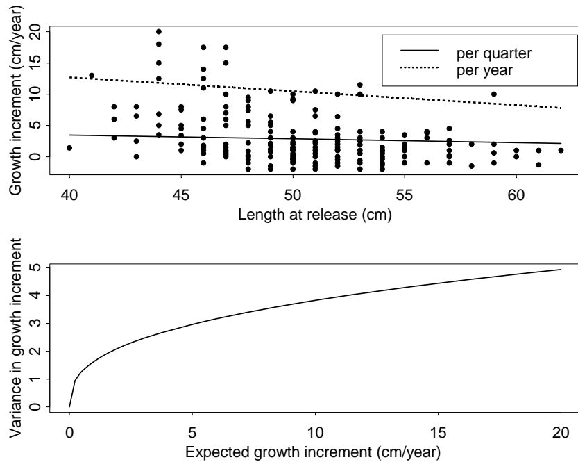
Figure 4. Expected growth increment from the alternative von Bertalanffy-Fabens's model for different lengths at release and times at liberty: one year and a quarter (top). Changes in growth variability over the growth increment as described by the Francis variance model C (bottom).
