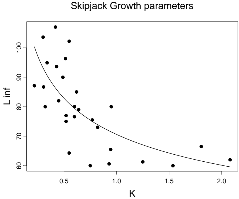
Figure 2. Distributions of combinations of estimates of L_{\infty} and K for skipjack tuna from different studies.
