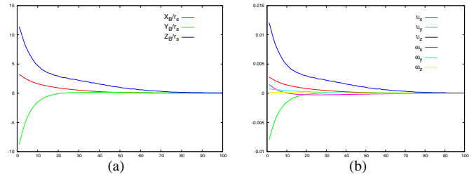
Fig. 8. Calibration errors \hat{p}_x > 0 & \hat{p}_y > 0 . (a) \frac{\mathbf{B}}{r_s} error. (b) Computed camera velocities (m/s and dg/s).
