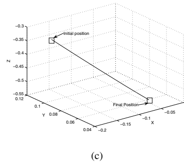
Fig. 5. Ideal case. (a) \frac{B}{r_s} error. (b) Computed camera velocities (m/s and dg/s). (c) Camera trajectory in the cartesian space.
