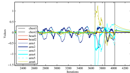
Fig. 5. Experiment B: Joint velocities. To improve the readability, only the joints of the chest, the head and the arm are given.
