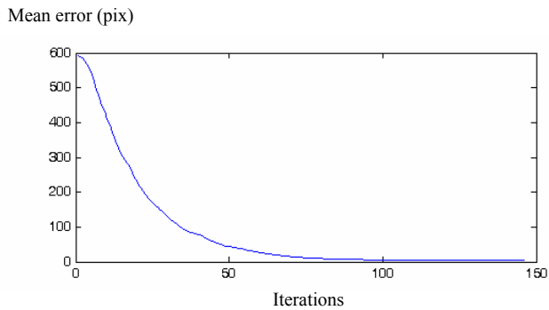
Fig. 7. Mean error in pixel. Test 2.
