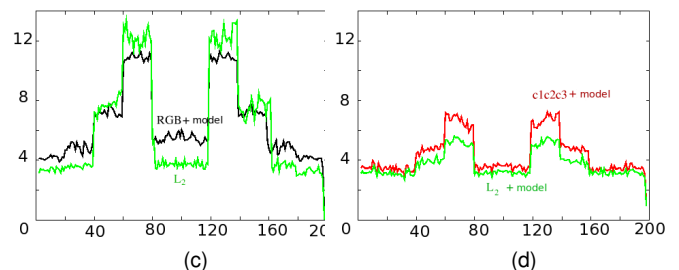
Fig. 5. Sequence 4 (a) : two images of the sequence. (b) : number of points which are correctly tracked (on 15 points initially selected). (c) and (d) : convergence residuals obtained with \mathcal{N} = 15 .
