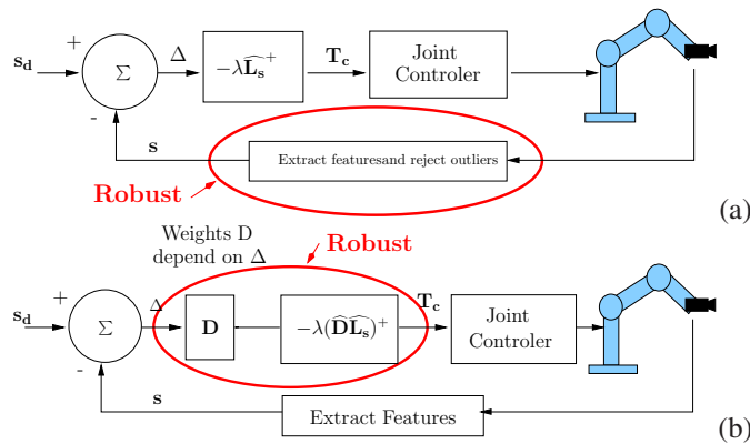
Fig. 10. Visual servoing with (a) traditional outliers rejection process at the image processing level, (b) Outliers rejection within the control law
