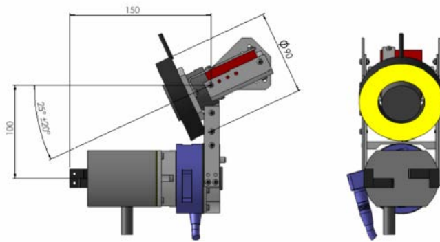
Figure 6: The VIMANCO Arm Camera Vision System
