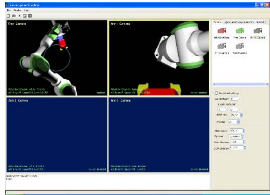
Figure 6: The VIMANCO Arm Camera Vision System
