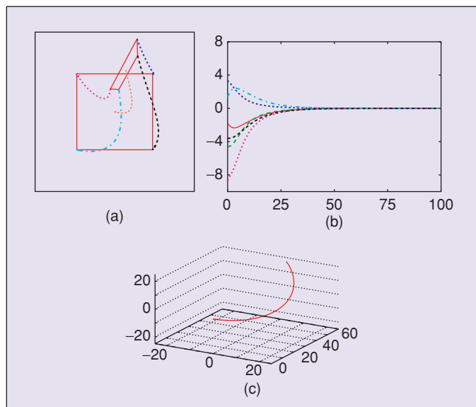
Figure 4. The system behavior using \mathbf{s} = (x_1, y_1, \dots, x_4, y_4) and \mathbf{L}_e^+ = \frac{1}{2}(\mathbf{L}_e + \mathbf{L}_{e^*})^+ .
